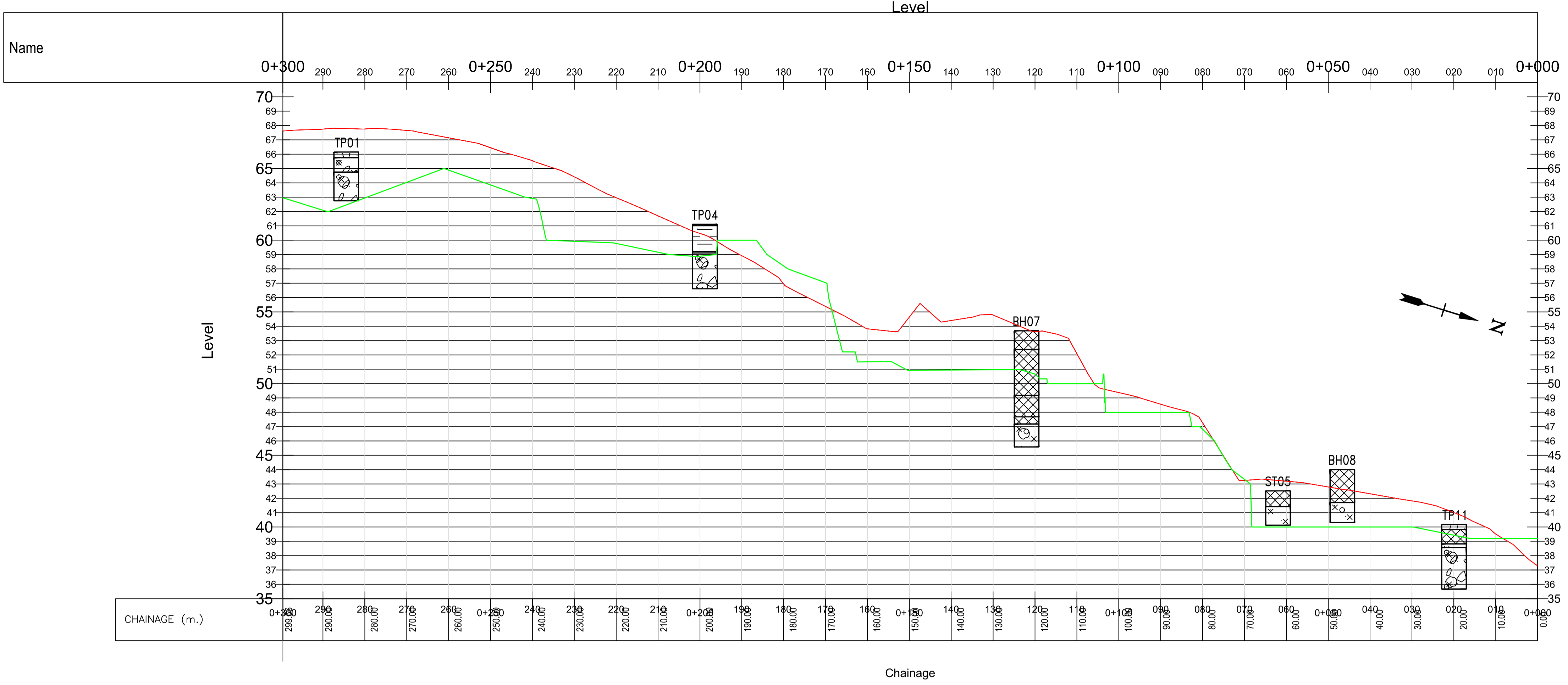
LONGSECTION OF BASELINE 1 - LONGSECTION 1 SCALE: H 1:500, V 1:146. DATUM: 35.000
